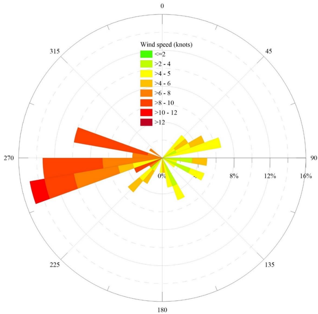
Figure 39: Windrose for Hanimaadhoo station 2012 to 2016
