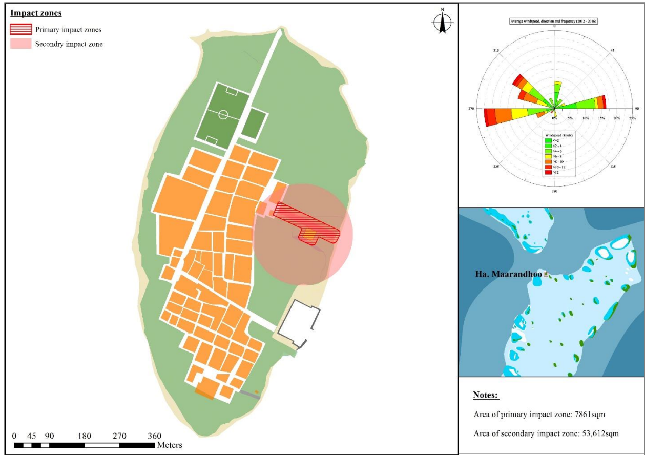
Figure 77: Primary and secondary impact zones Ha. Maarandhoo
