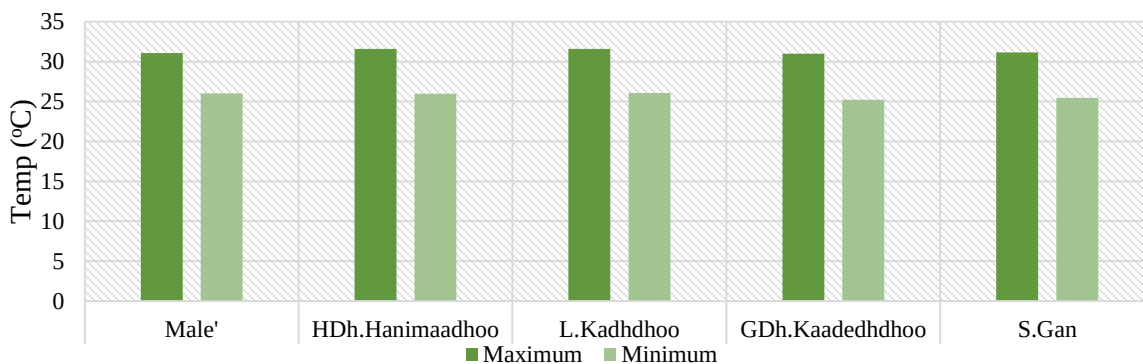
Figure 38: High and low temperature variance between atolls of the Maldives
