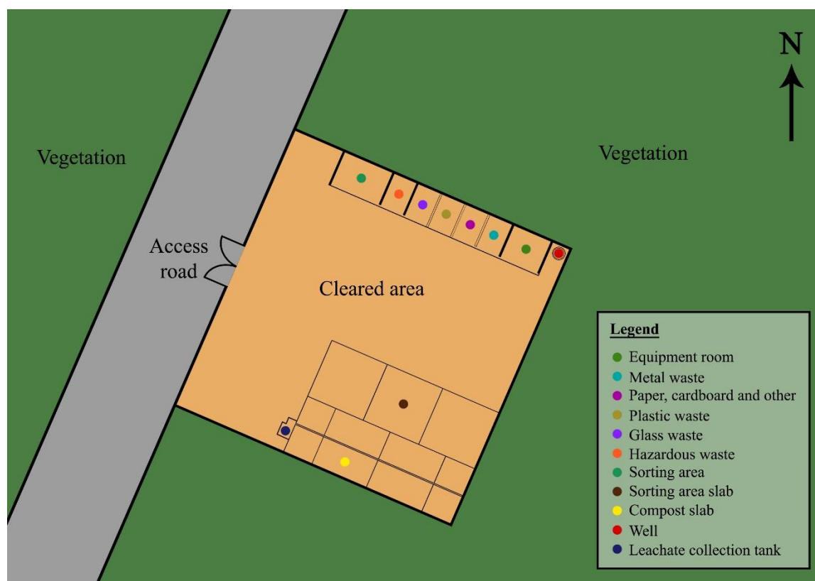
Figure 22: Typical plan of the IWMC center
