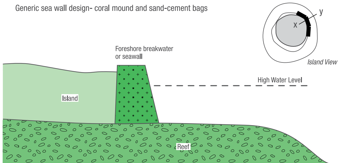
Figure 4.2 Generic sea wall design for coral mound, sand-cement bags, sheet and wooden piles
