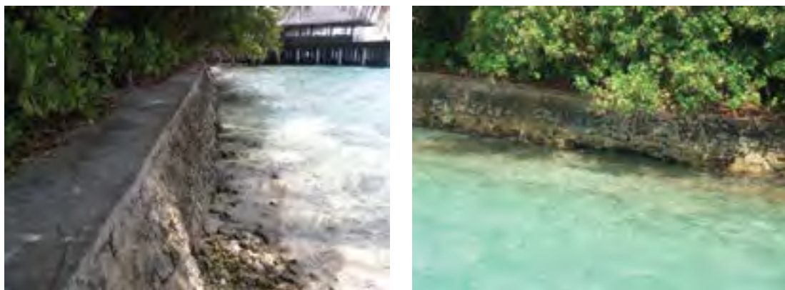
Figure 4.7 Examples of Seawall structures: semi-plastered coral mound seawall in Boduhithi
