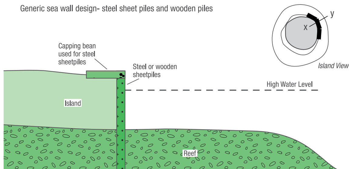
Figure 4.3 Generic sea wall design for coral mound and sand-cement bags
