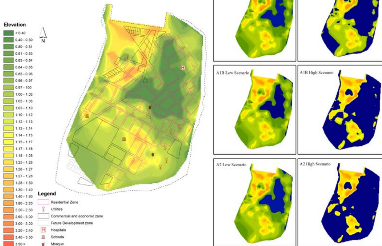
Figure 7-2: Inundation of Hithaadhoo island under future climate change scenarios
