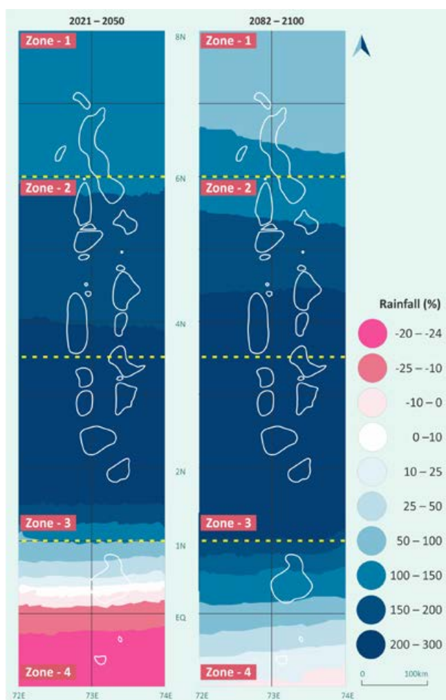
Figure 3-7: Changes in monsoonal rainfall from IPRC RegCM scenario for time slices (2021-2050) and (2082-2100) from baseline (1980-2000). Rainfall change for months MJJ-ASO in %. (adopted from MEE, 2015a)
