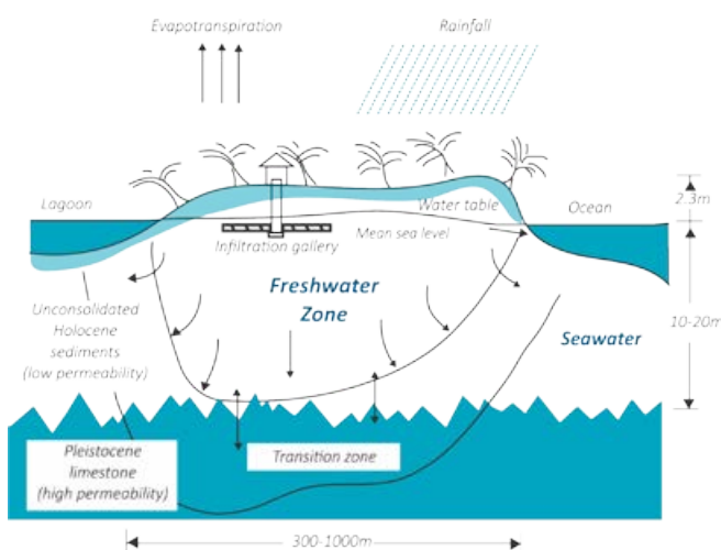
Figure 2-27: Schematic showing a typical water lens of an island (adapted from White et al., 2007)
