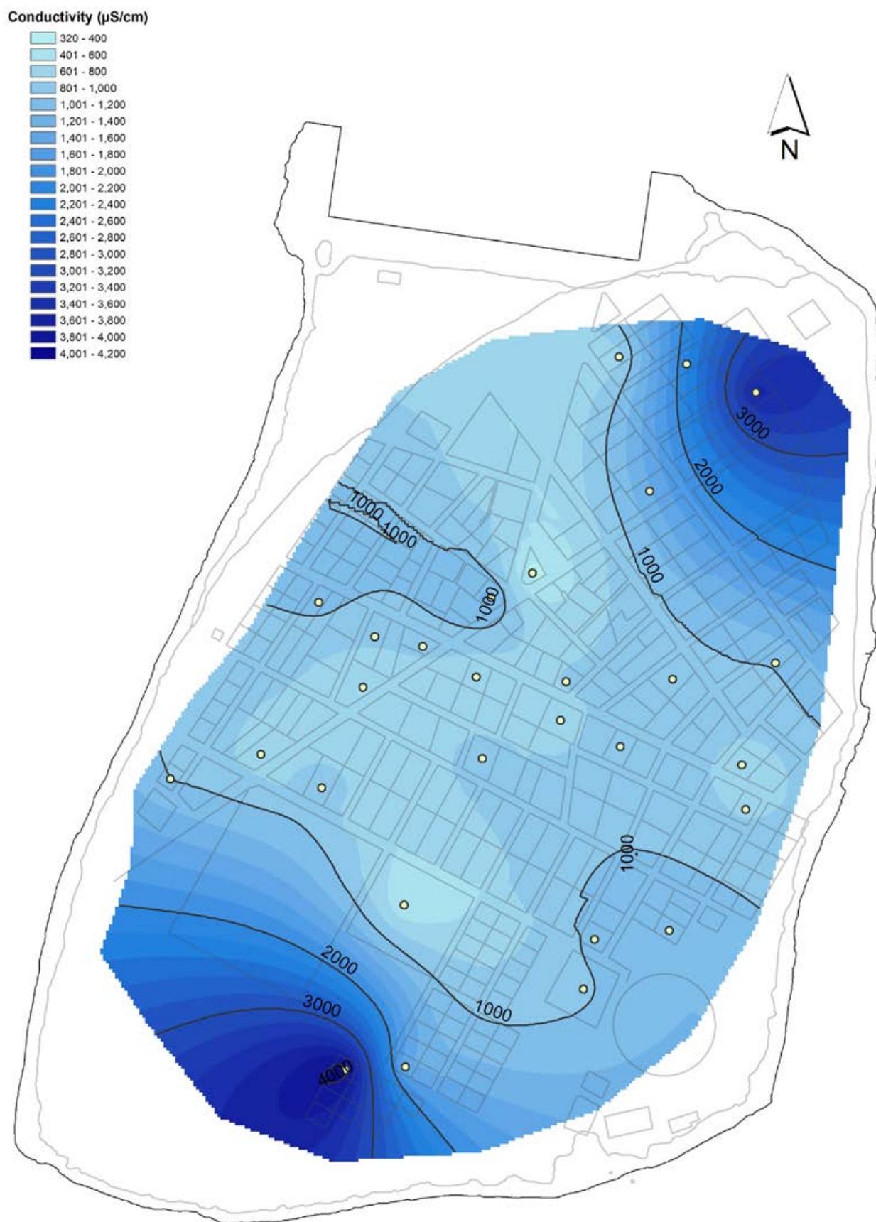
Figure 7-3: Electrical conductivity map of Baa Hithaadboo
