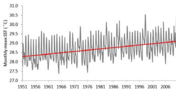
Figure 3-5: Sea surface trend in central Maldives (1951-2010) (data source: Rayner et al., 2003)
