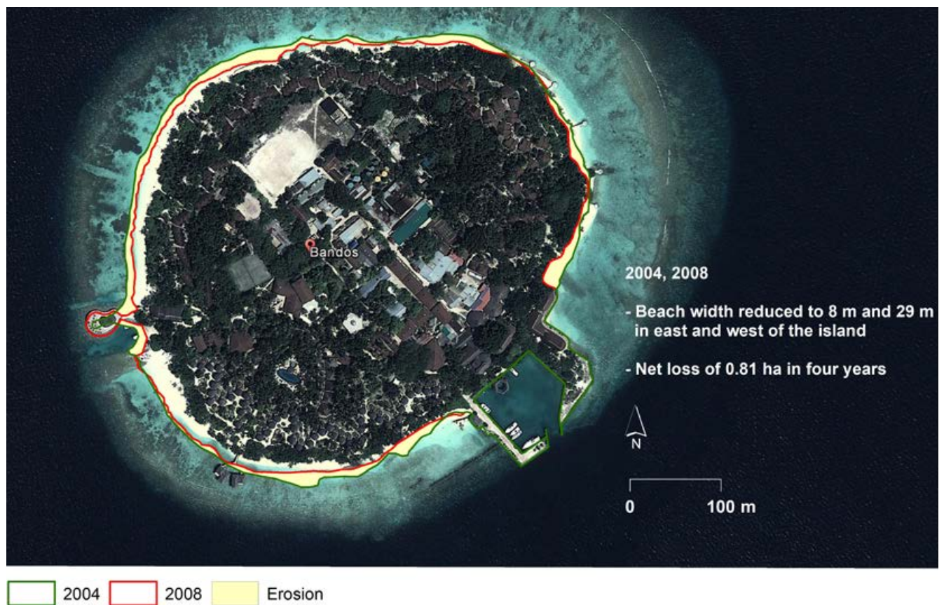
Figure 7-1: Shoreline analysis of the case study islands showing net erosion and accretion zones (images: Google Earth).
