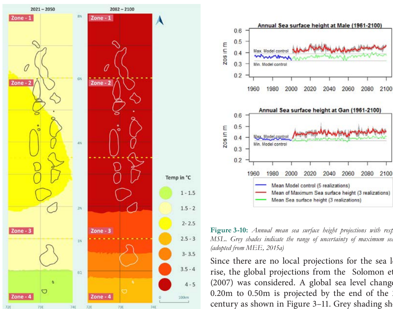
Figure 3-9: Changes in temperature from IPRC RegCM scenario for time slices (2021-2050) and (2082-2100). Baseline is (1980-2000). Temperature change for months MJJASO in degree Celsius. (adapted from MEE, 2015a)
