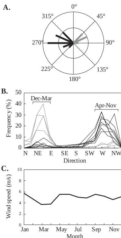
Figure 11. Summary of wind data for the Maldives showing A) 30-year mean percent frequency wind direction B) 30-year mean monthly percent frequency wind direction; C) 30-year mean monthly wind speed. Climate data from Government of Maldives, Department of Meteorology, (1995) adapted from Kench et al; (2010).
