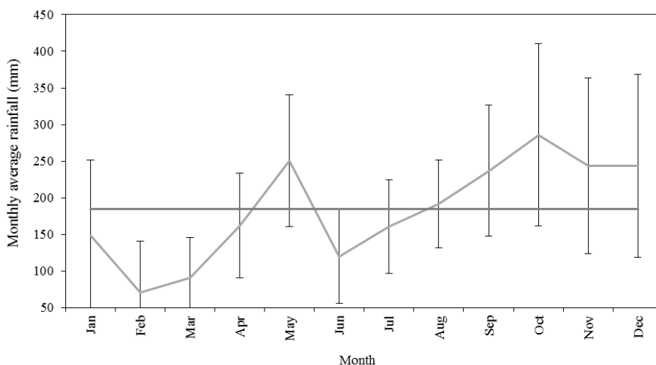
Figure 10. Average rainfall for the twelve months of the year for Kadhdhoo Island (1992-2013). (The solid dark grey line indicates monthly average).
