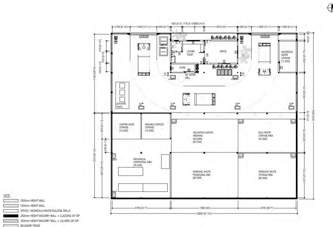
Figure 4: Site Plan for IWRMC in Th. Omadhoo
