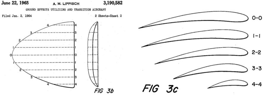
Figure 8. The wing shape is half of an ellipse. The wings are highly under-cambered.
