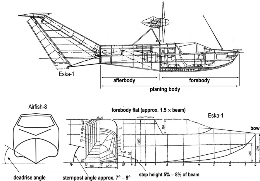
Figure 10. Common terms used in WIG design.
