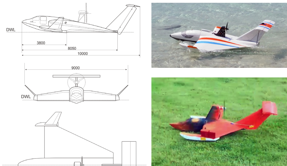
Figure 11. Dimensions of the full-scale WIG craft. The one-sixth scale model is shown on the right above. Below that is a one-seventh scale model with Clark-Y airfoil used in an earlier investigation.
