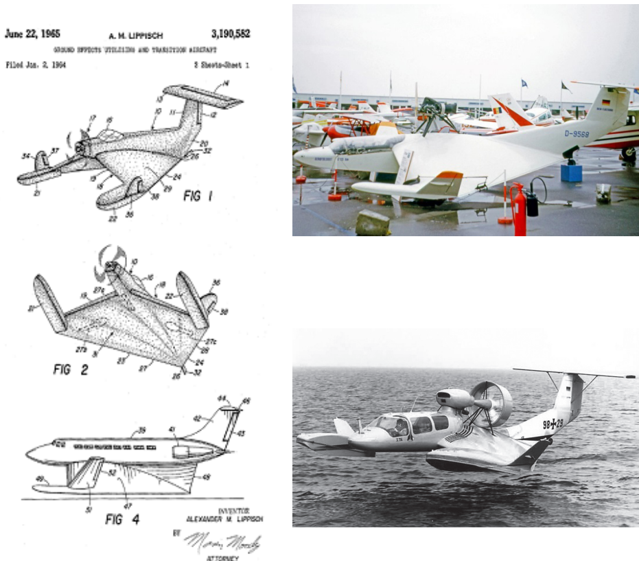
Figure 1. On the left is the original drawings of the Lippisch patent for the WIG craft. On the right at the top is X-113, and below it is X-114.
