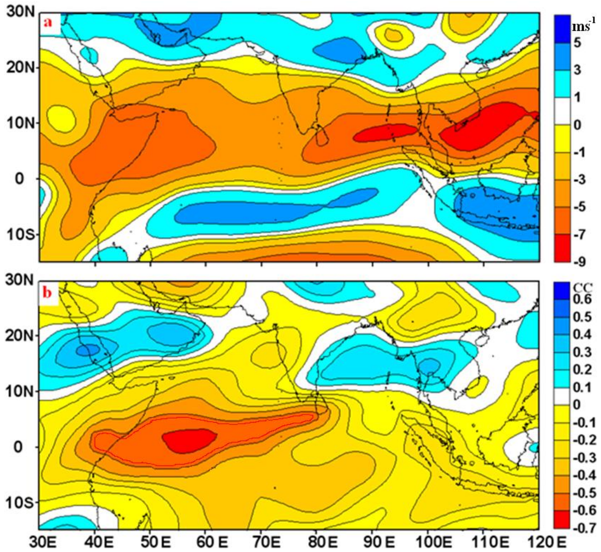
Figure 5.6: 850 hPa mean zonal wind (m/s) for January (a) and correlation between JJAS total precipitation over the Maldives and 850 hPa mean zonal wind for January (b), from 1979 to 2007. The red contour lines indicate areas of significant correlation (1% level). The negative/positive values of zonal wind indicates easterly/westerly direction, respectively.
