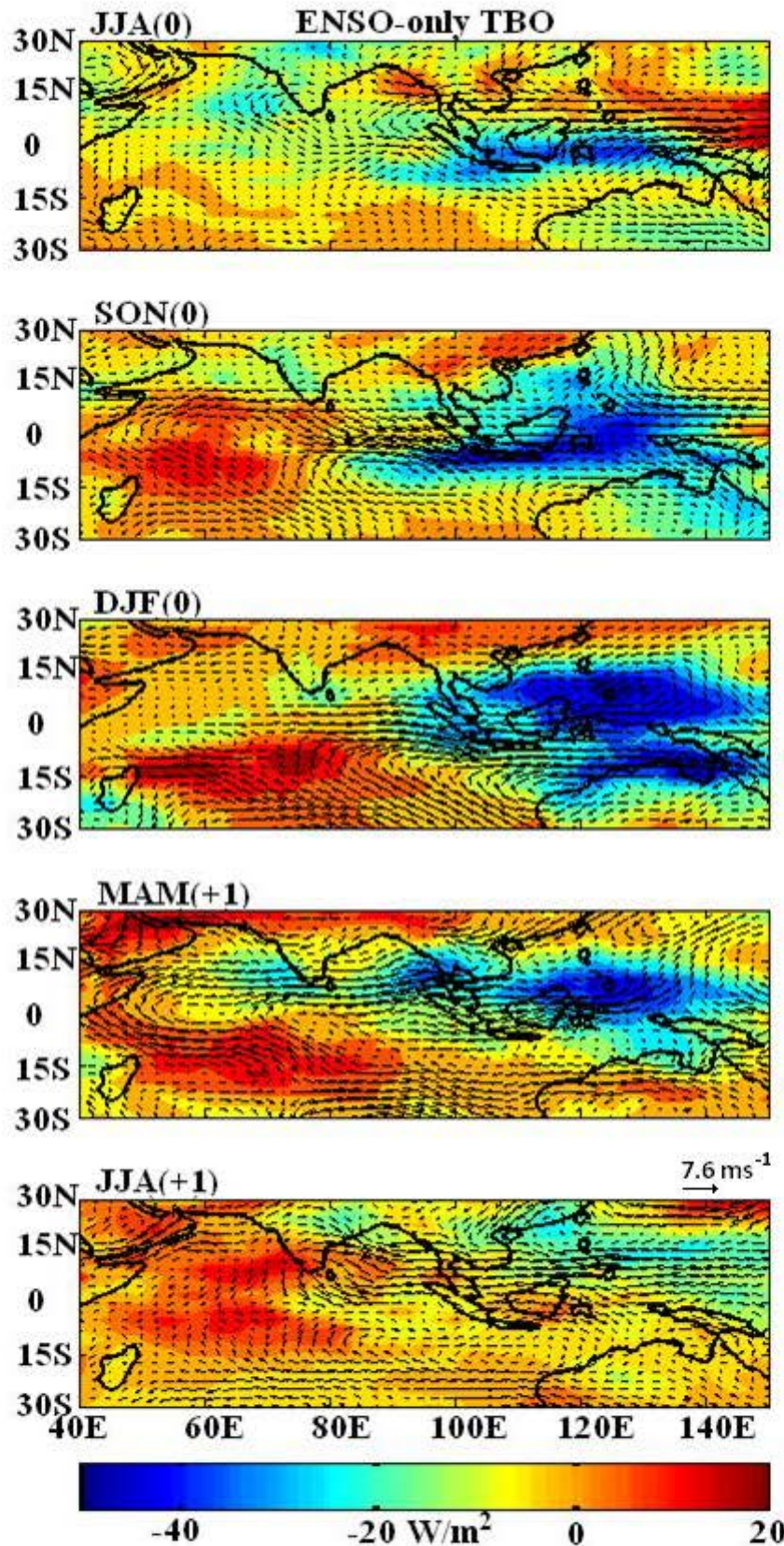
Figure 7.17: Strong minus weak ENSO TBO composites of outgoing longwave radiation (OLR: shaded) and 850 hPa wind (arrows: key is indicated at the bottom plot), starting from strong monsoon, JJA (0), to the next year monsoon, JJA (+1).
