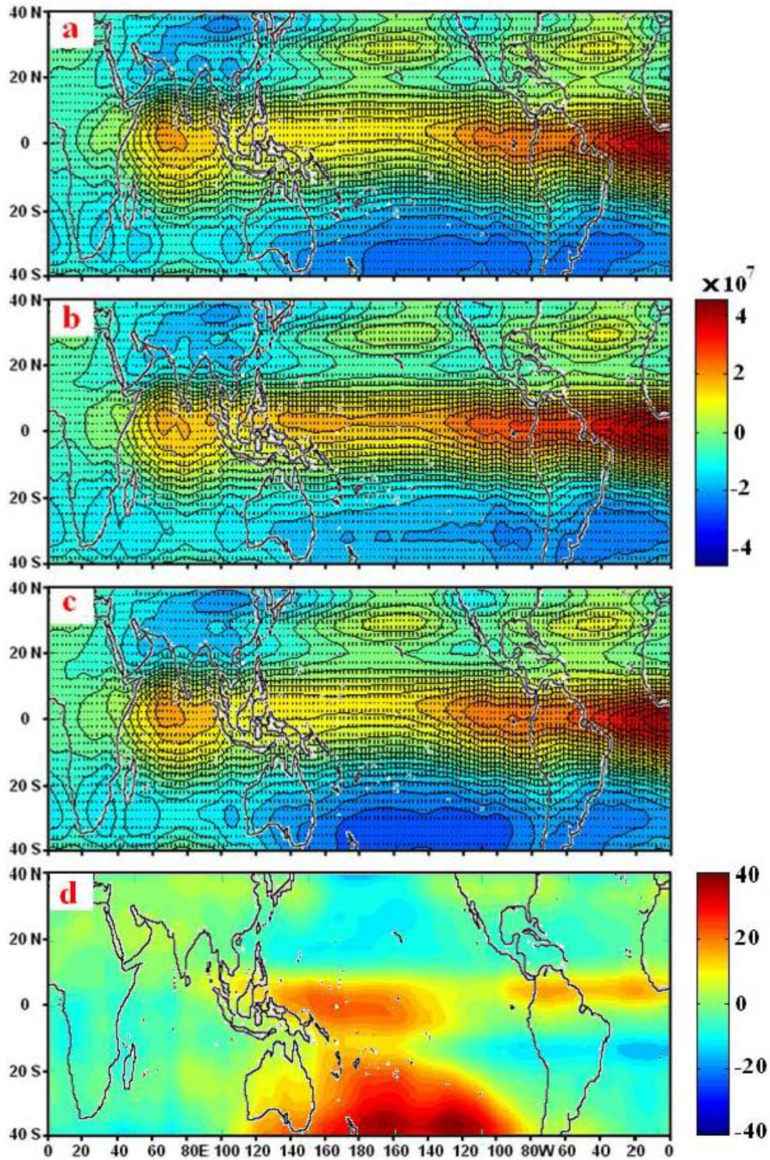
Figure 6.13: 850 hPa June-September mean velocity potential ( \text{m}^2/\text{s} : contour shadings) and divergent wind ( \text{m/s} : arrows) for: (a) Non-ENSO years, (b) El Niño deficient monsoon rainfall years (1987, 1991 and 2002), (c) La Niña excess monsoon rainfall years (1988, 1998 and 2007) and (d) Difference between El Niño years and La Niña years (b minus c) velocity potential magnitude ( \text{m}^2/\text{s} ).
