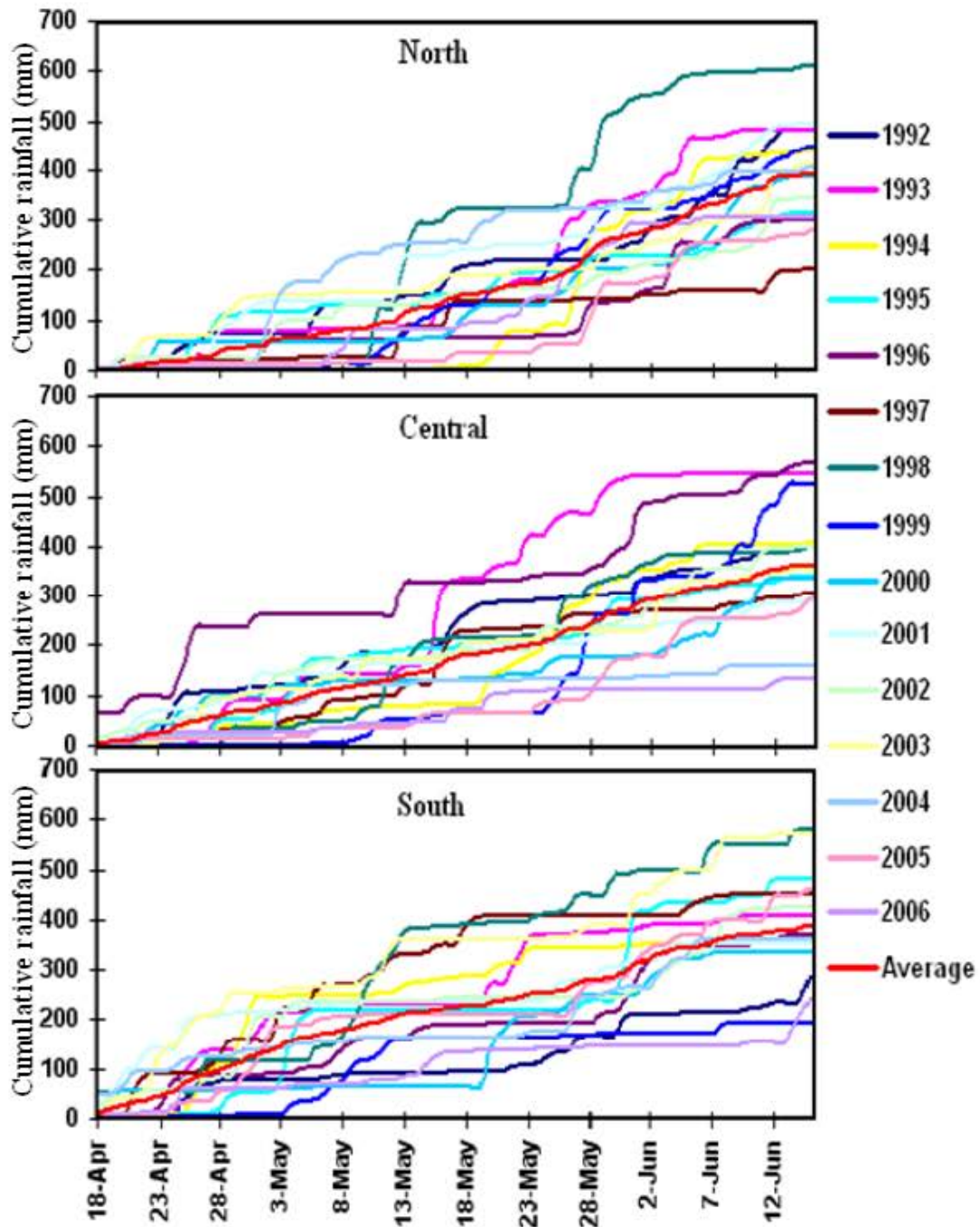
Figure 4.44: Cumulative daily total rainfall for the onset phase of the monsoon from 1992 to 2006 for the north, central and southern parts of the Maldives.
