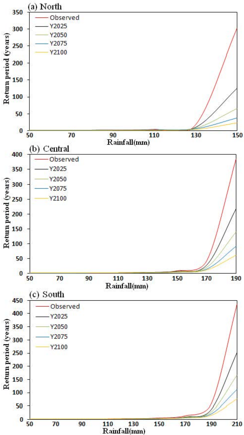
Figure 8.3: Observed and predicted (for years 2025, 2050, 2075 and 2100) return periods for: (a) northern, (b) central and (c) southern Maldives regions based on daily rainfall for the periods 1992-2009 (northern), 1975-2009 (central) and 1980-2009 (southern).
