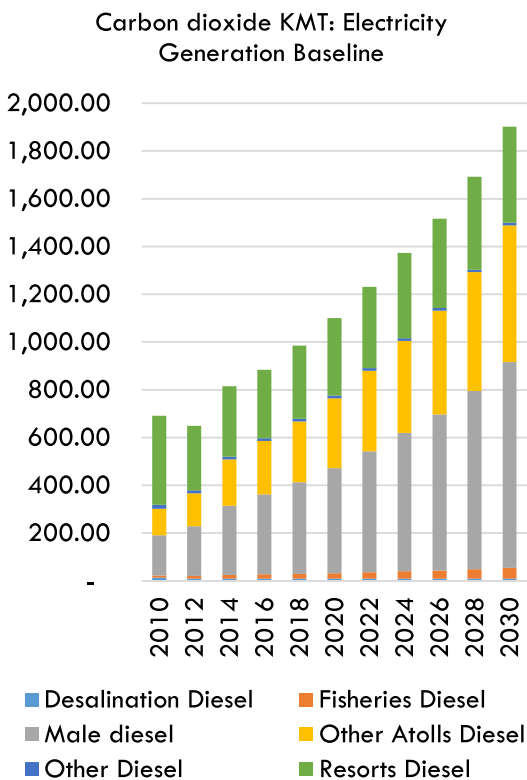
FIGURE 12: PROGRESSION OF CARBON DIOXIDE EMISSIONS FROM ELECTRICITY GENERATION.
