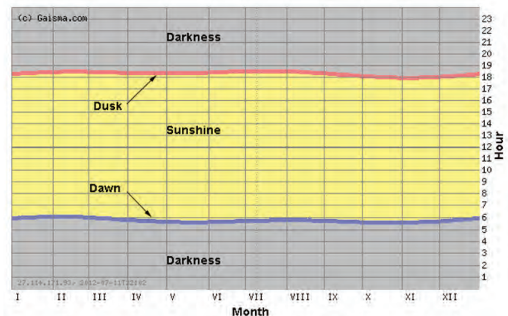
Figure 13: Solar insolation in Male' (source: www.gaisma.com )
