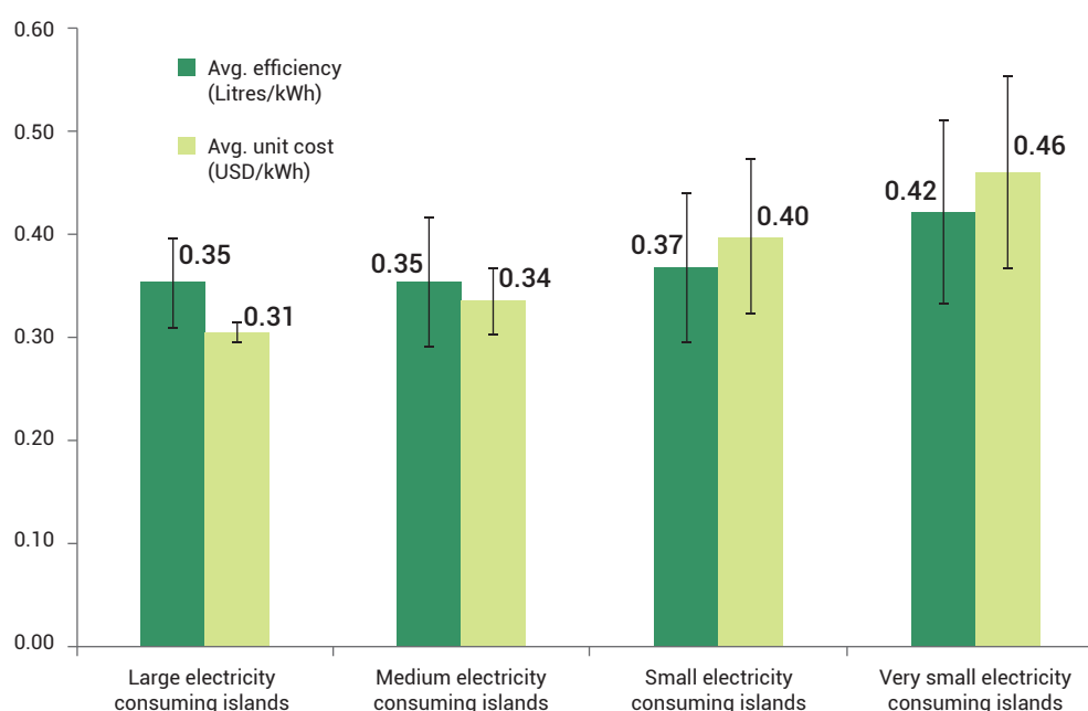
Figure 8: Comparison of average fuel efficiency and unit cost of generation for the different categories of outer islands 15
